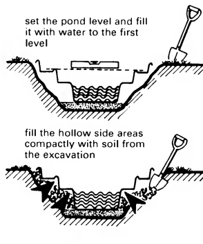
④ Garden pond installation: compacting
